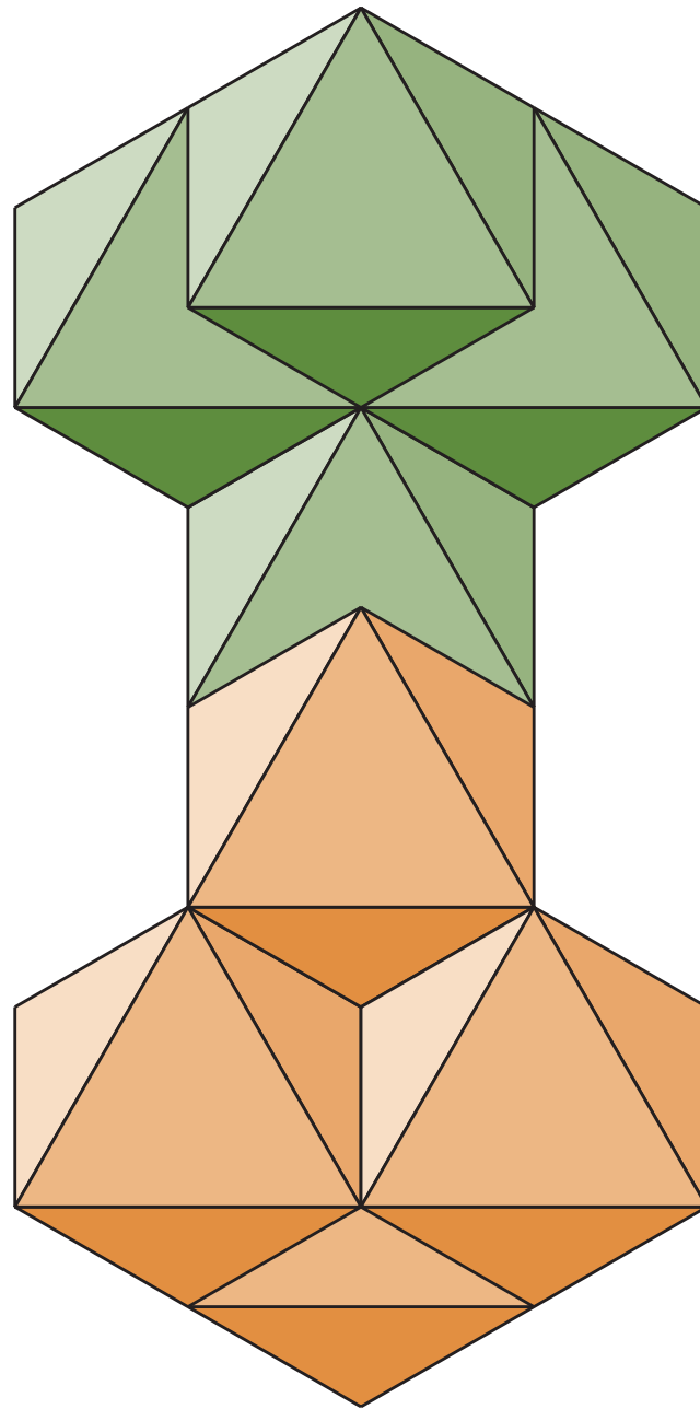
O-O join
