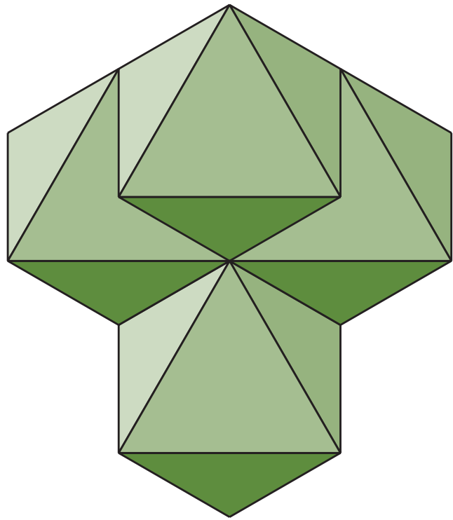
O-atom
