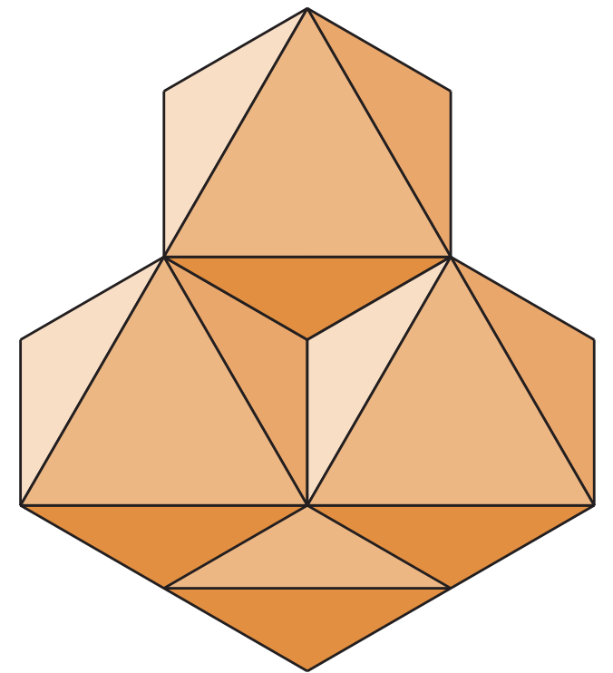
O-atom
