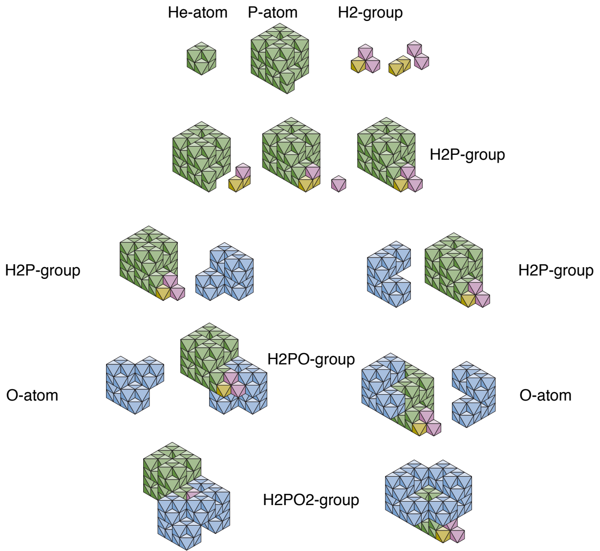
Figure 6: Steps in the assembling of the \text{H}_2\text{PO}_4 -group
