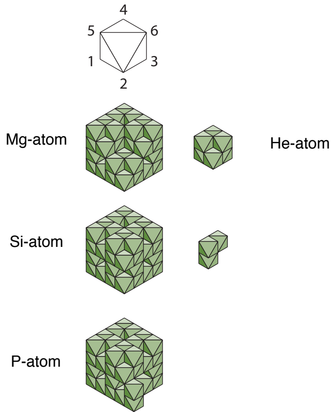
Figure 1: The P-atom
