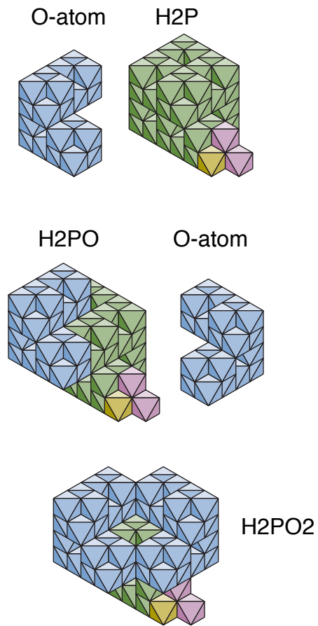
Figure 5. Attaching O-atoms to the Na/Si-octa of the P-atom.
