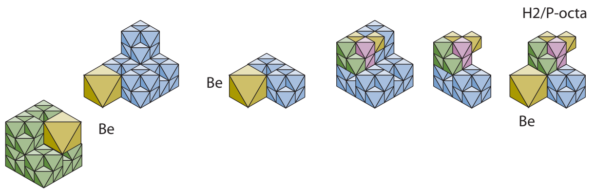
Figure 5: Cleft join of the O-atom with the P-atom within H 2 PO-group-1.
