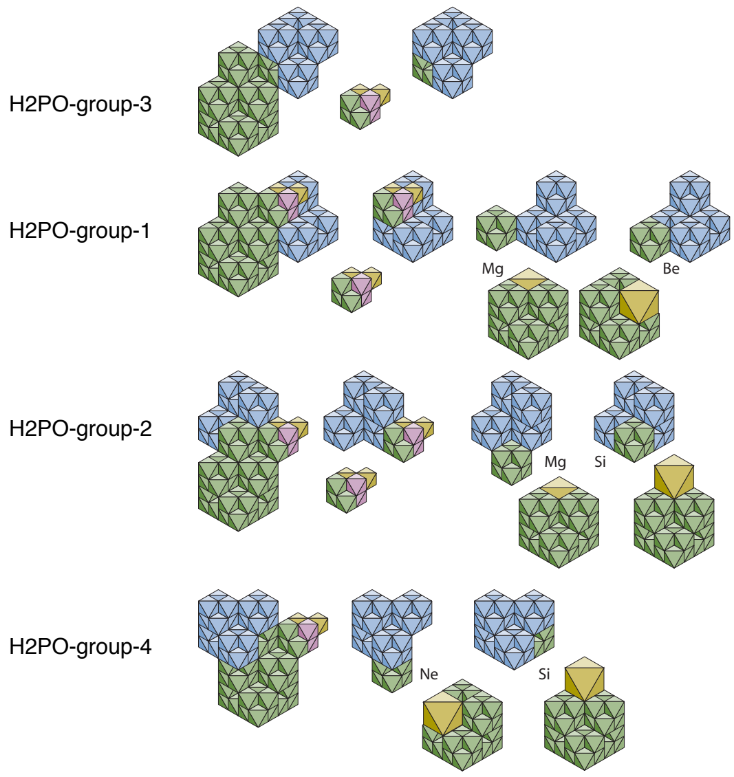
Figure 3: Examination of the attachments between the parts of the P-atom and each of the four O-atoms of the H 2 PO 4 -group.
